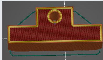
Infill 90%
